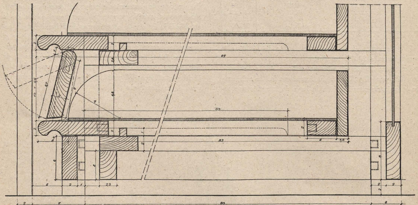
DETALLE (A)
