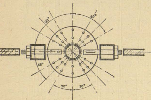
SOPORTE-LIMBO PERFORADO (PLANTA DETALLE 5)
