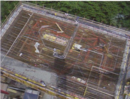
Distintos momentos del proceso constructivo. Different moments during the building process.
